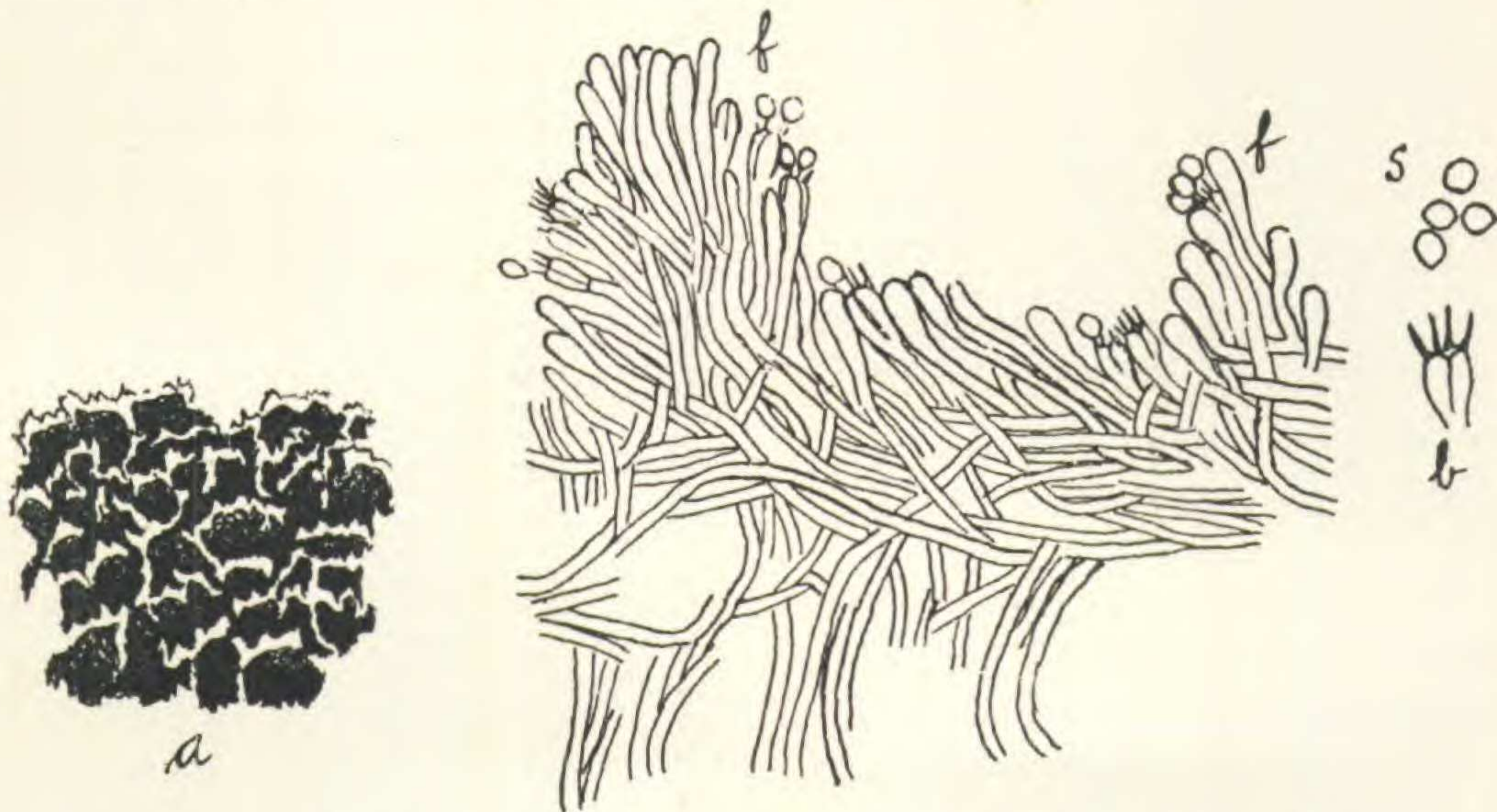
Fig. 1. P. Farlowii . a , fructification viewed from above, showing pores in black and folds and dissepiments in white, \times 68 ; f and f , section of fructification showing pore between folds, \times 375 ; b , basidium, and s , spores, \times 375 .
